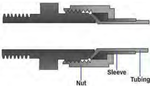
Figure 9-28 – Flared-tube connector.
